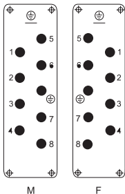
接插针排序/Contact arrangement view from termination side
