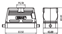
低结构/Low construction
