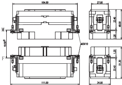
接插针排序/Contact arrangement view from termination side
