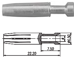
插孔/Female
