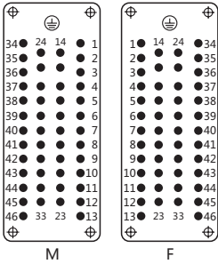
接插针排序/Contact arrangement view from termination side
